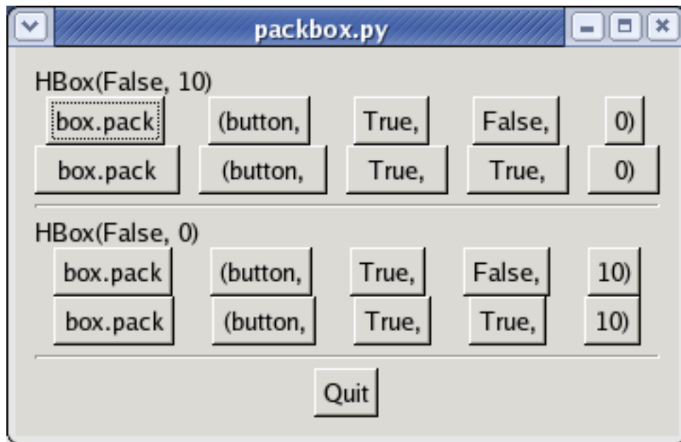
Figure 4.2. Packing with Spacing and Padding
