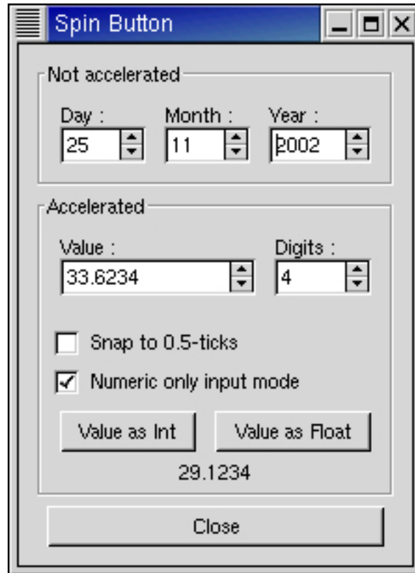
Figure 9.11. Spin Button Example
