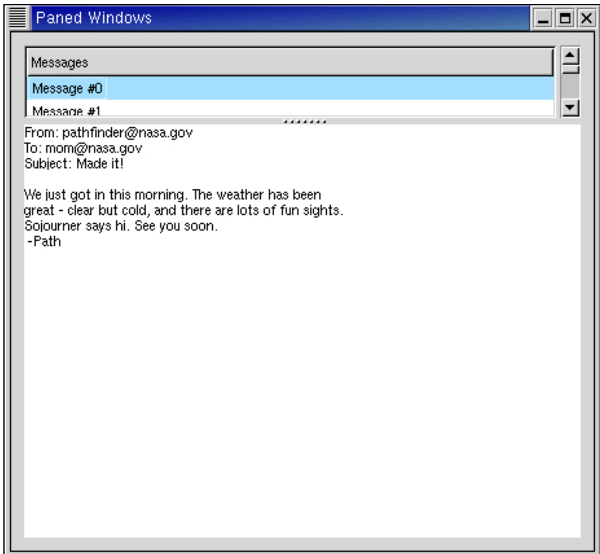
Figure 10.6. Paned Example
