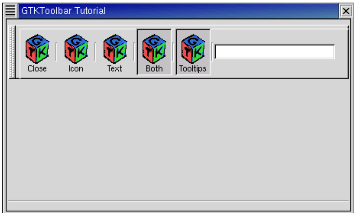
Figure 10.8. Toolbar Example
