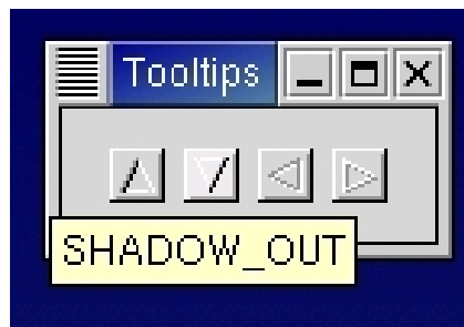
Figure 9.3. Tooltips Example
