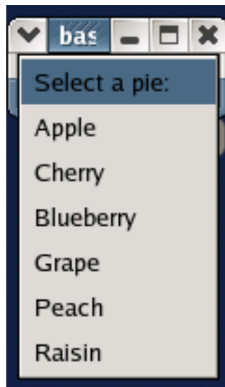
Figure 16.5. Basic ComboBox
