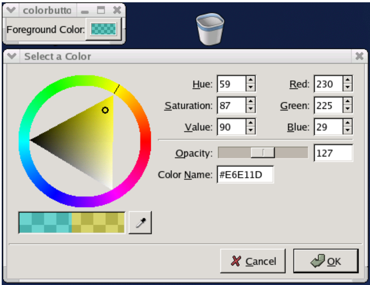
Figure 16.8. ColorButton Example
