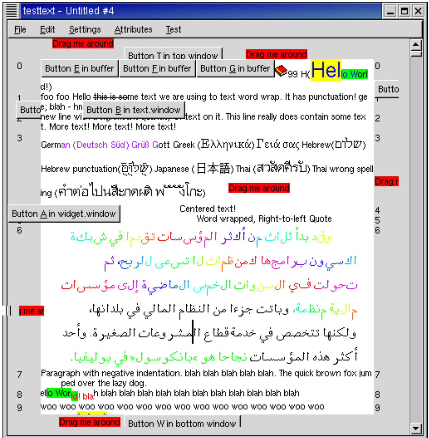
Figure 13.2. TextView Example
