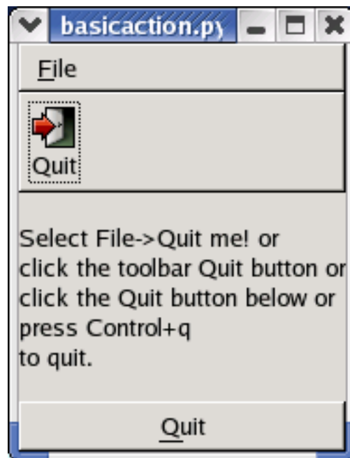
Figure 16.2. Basic Action Example
