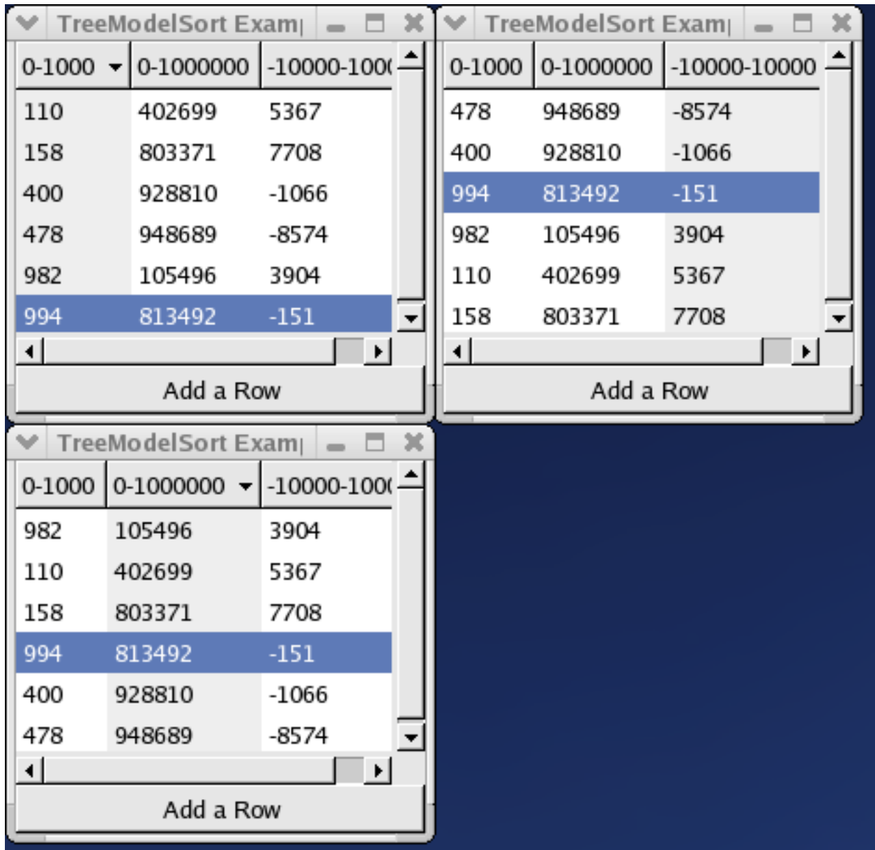
Figure 14.9. TreeModelSort Example
