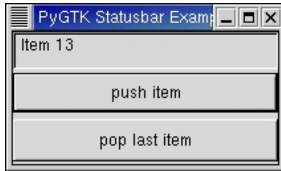
Figure 9.9. Statusbar Example
