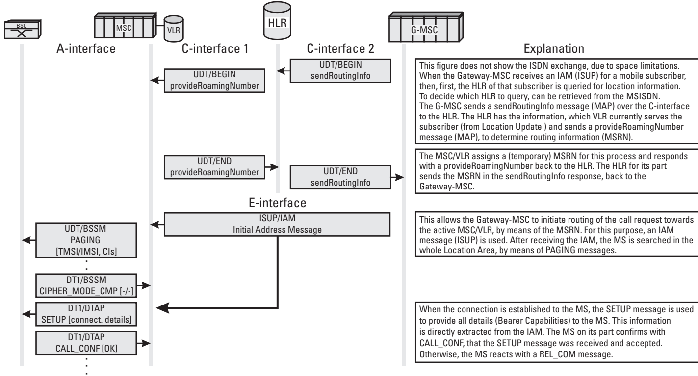
Figure 12.9 Mobile terminating call in the NSS.
