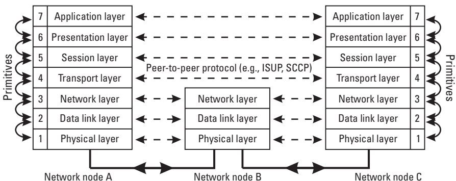
Figure 5.1 The layers and message types of the OSI Reference Model.
