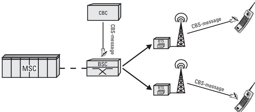
Figure G.13 Function of the CB/SMSCB.
