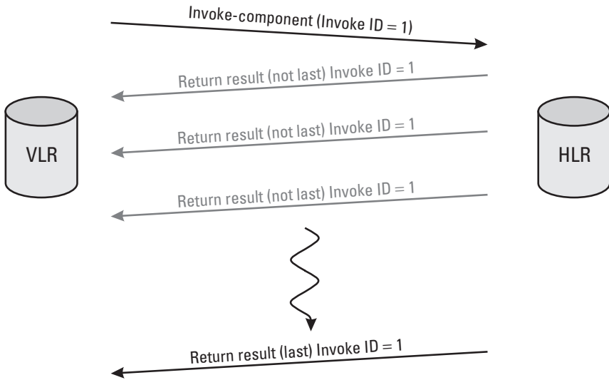
Figure 11.17 Use of the return result ( last ) and ( not last ) components.
