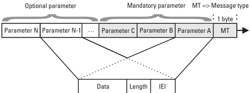
Figure 10.5 The internal structure of BSSMAP messages.
