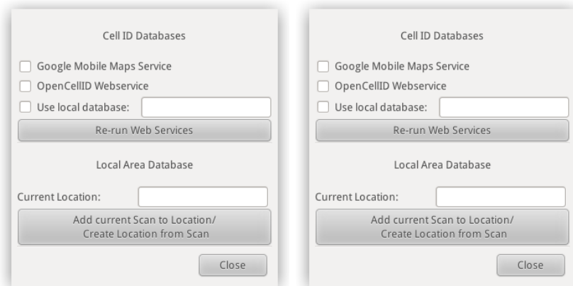
(a) Databases window.
