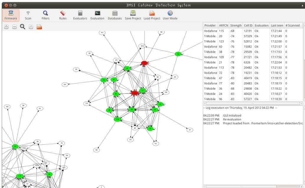
Figure 3.7.: The ICDS main window.
