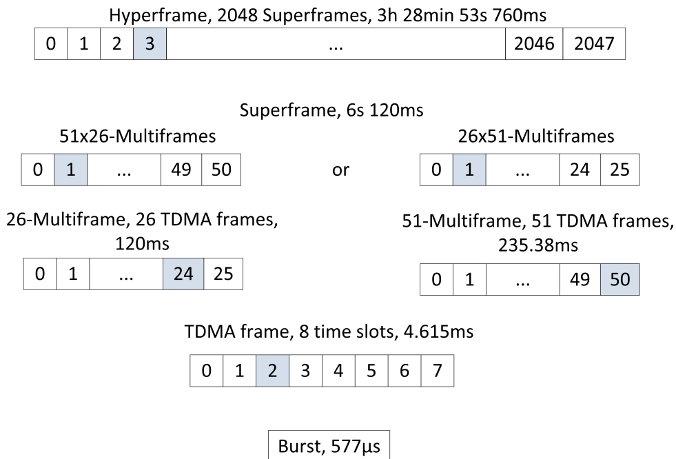
Figure 2.8.: Hierarchical Composition of the different frames.
