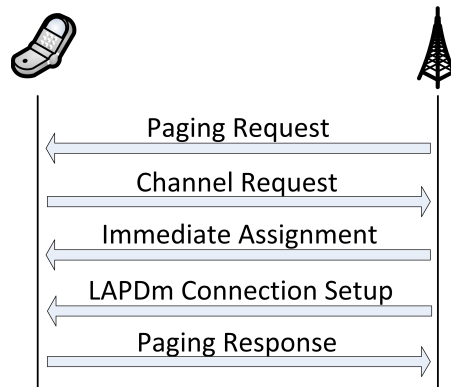
Figure 3.6.: Procedure taken when the network has a call/text waiting for a passive subscriber.
