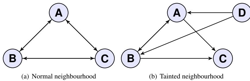
Figure 3.5.: Comparison between a normal neighbourhood subgraph and a tainted one.
