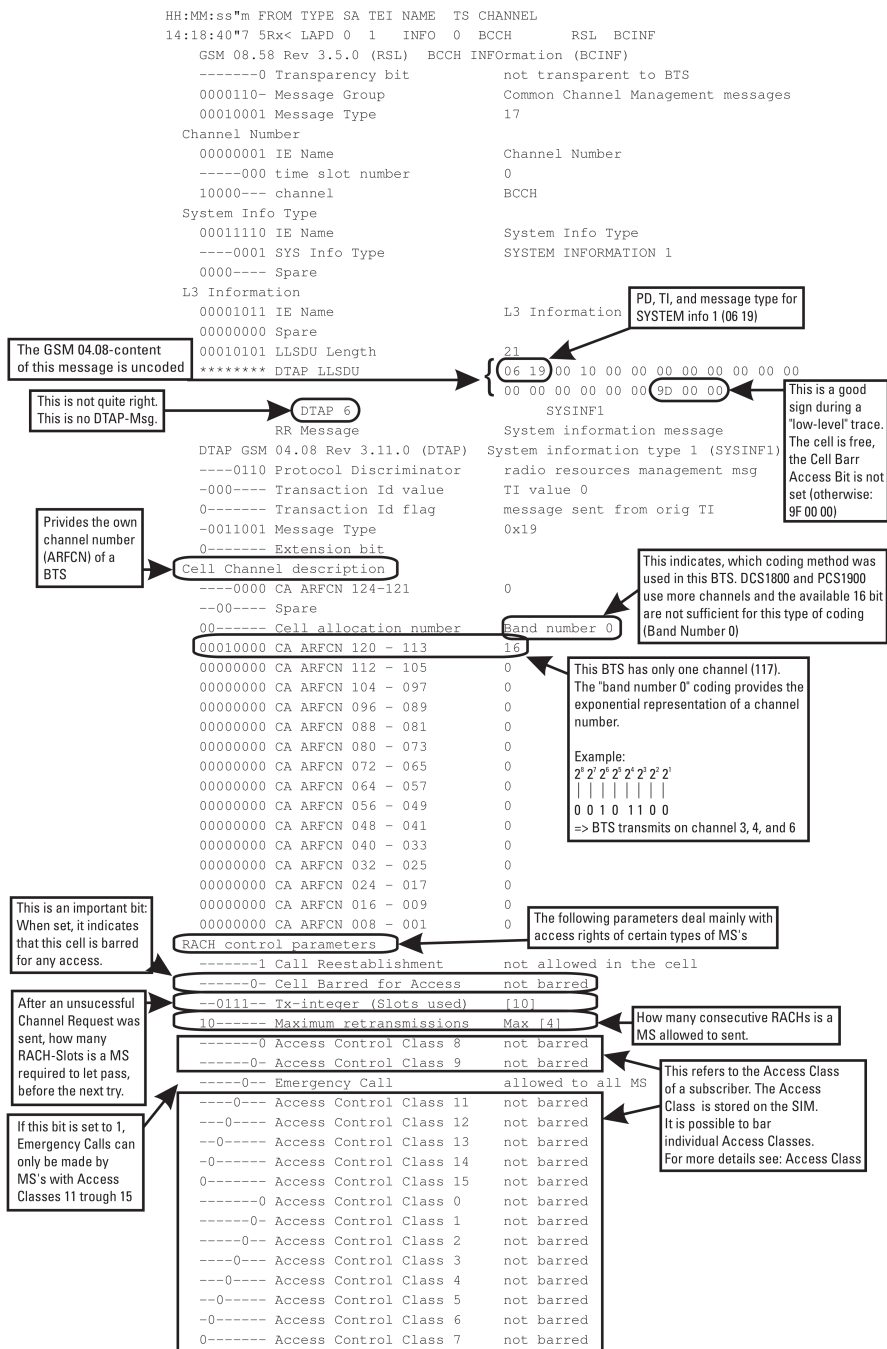
Figure 3.3.: System Information 1 Message [17].
