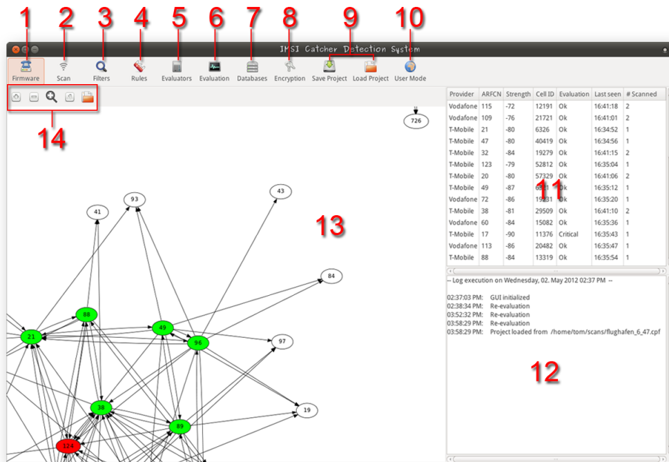
Figure 3.8.: The ICDS main window.
