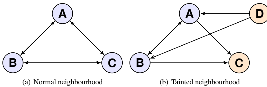
Figure 3.6.: Comparison between a normal neighbourhood subgraph and a tainted one.
