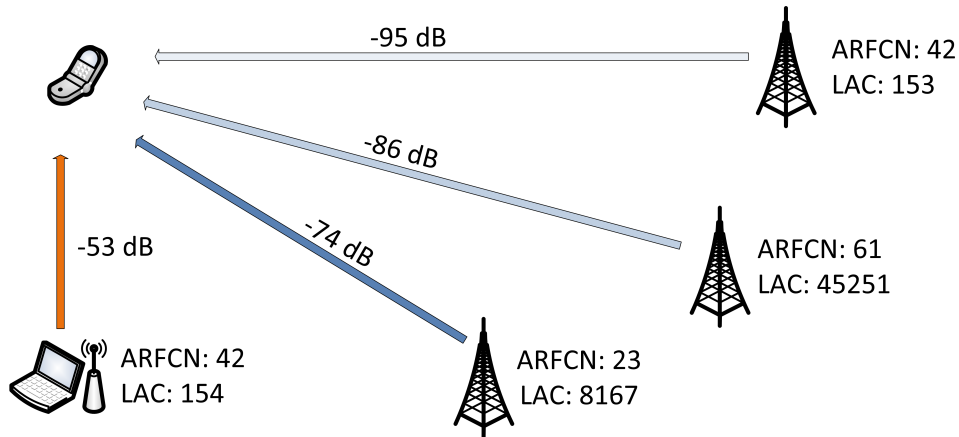
Figure 4.5.: Takeover attack of an IMSI catcher on a base station.
