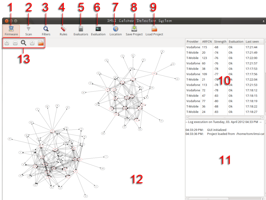
Figure 3.7.: The ICDS main window.
