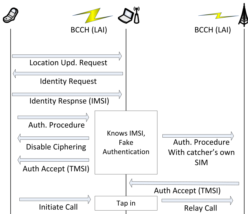
Figure 2.12.: IMSI catching procedure. Adopted and simplified from [12].
