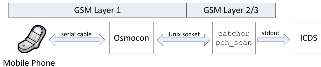
Figure 3.2.: Interaction of the OsmocomBB components with the ICDS software.
