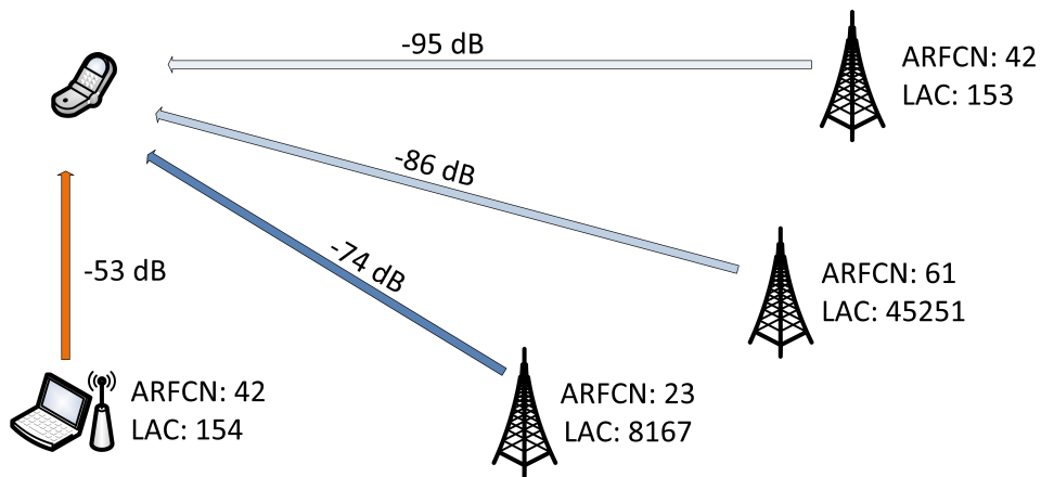
Figure 4.4.: Takeover attack of an IMSI catcher on a base station.
