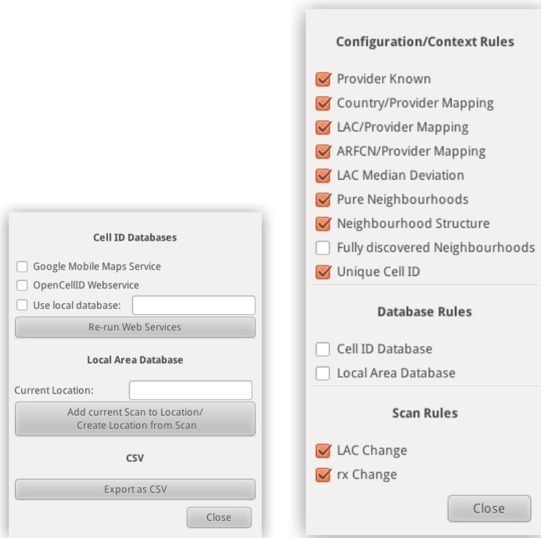
(a) Databases window.
