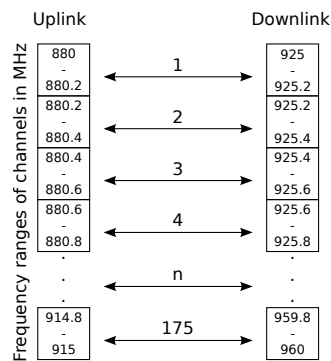
Figure 2.2.: Frequency ranges of uplink and downlink channels in the GSM900 band. Each box represents a frequency band (channel). Image courtesy of [57] and [81].
