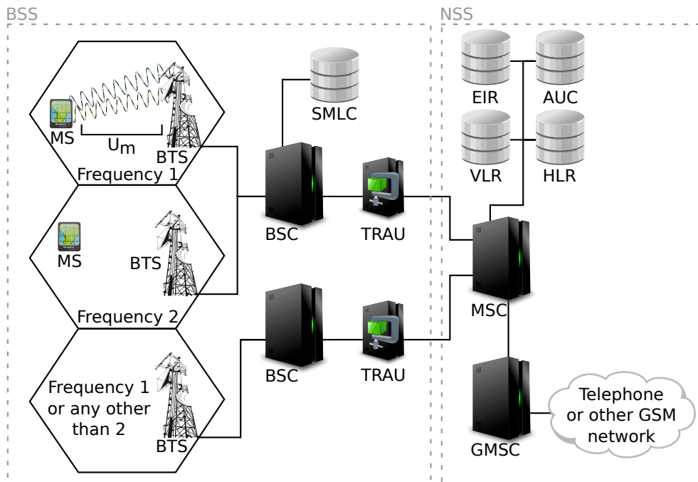
Figure 2.1.: Basic GSM network block diagram. Image courtesy of [57] and [81].
