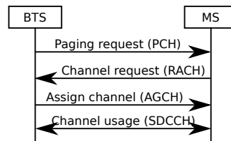
Figure 2.5.: Initializing an SDCCH channel. Image courtesy of [32].
