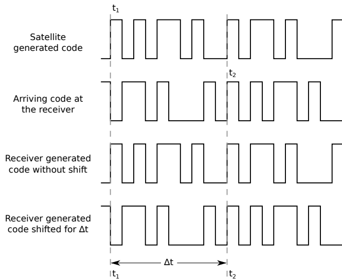
Figure 2.12.: Estimating the distance by phase shift \Delta t = t_2 - t_1 = \tau
