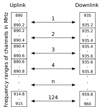
Figure 2.2.: Frequency ranges of uplink and downlink channels in the GSM900 band. Each box represents a frequency band (channel). Image courtesy of [57] and [80].
