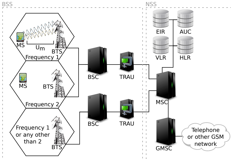
Figure 2.1.: Basic GSM network block diagram. Image courtesy of [57] and [80].
