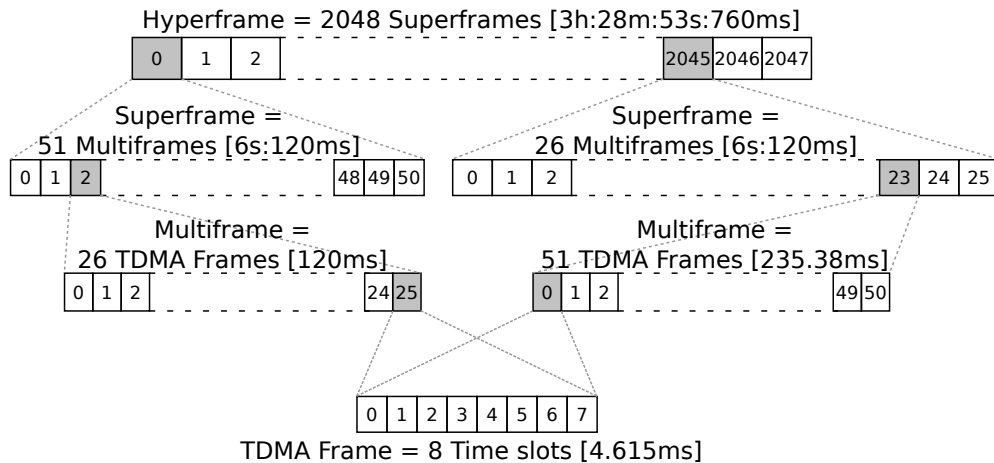
Figure 3.3.: Hierarchy of the frames in GSM.
