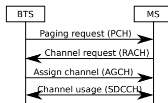
Figure 2.5.: Initializing an SDCCH channel. Image courtesy of [35].
