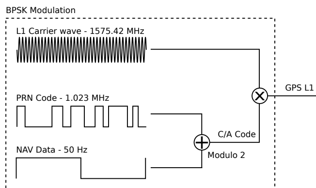
Figure 3.5.: Modulation of the GPS signal L1. Image courtesy of [37].
