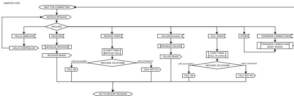
Figure 16: Flowchart of the protocol on the handler side without the state representation
