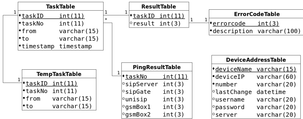
Figure 4: Database relationship diagram
