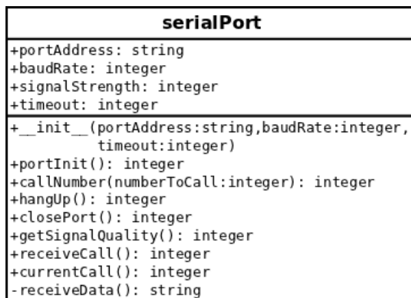
Figure 2: GSM class diagram for controlling the cell phones
