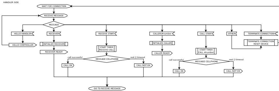
Figure 11: Flowchart of the protocol, on the handler side
