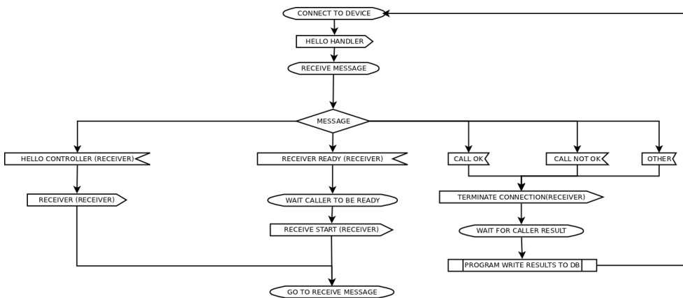
Figure 12: Flowchart of the protocol, on the controller side for the caller
