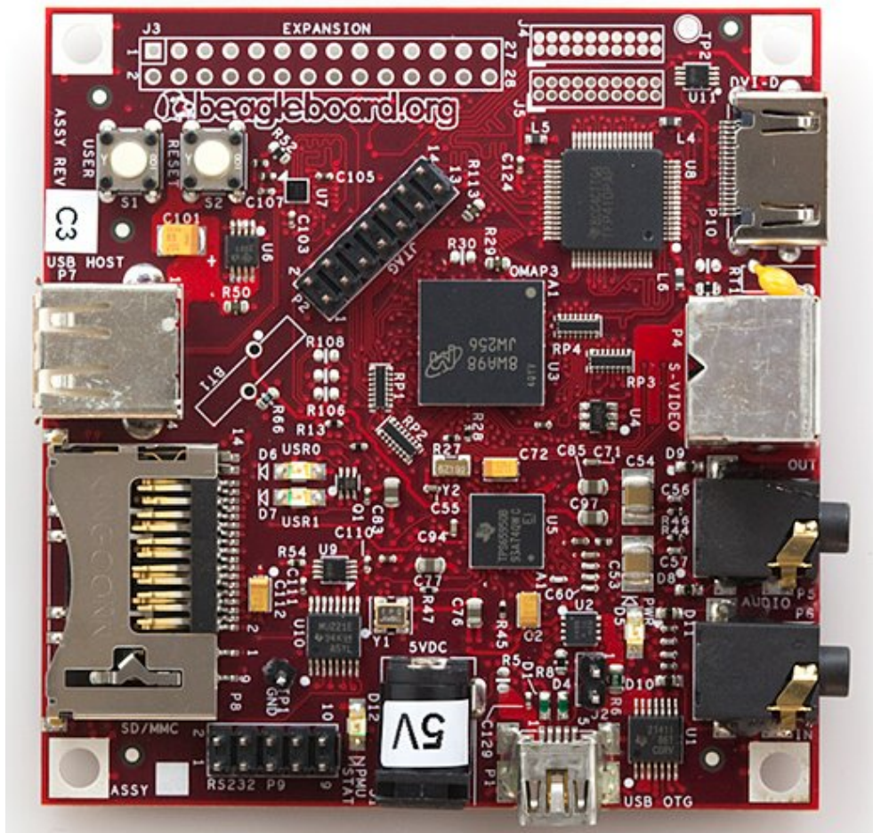
Figure 10: BeagleBoard, a Linux-on-chip board where our controller software runs the GSM device
